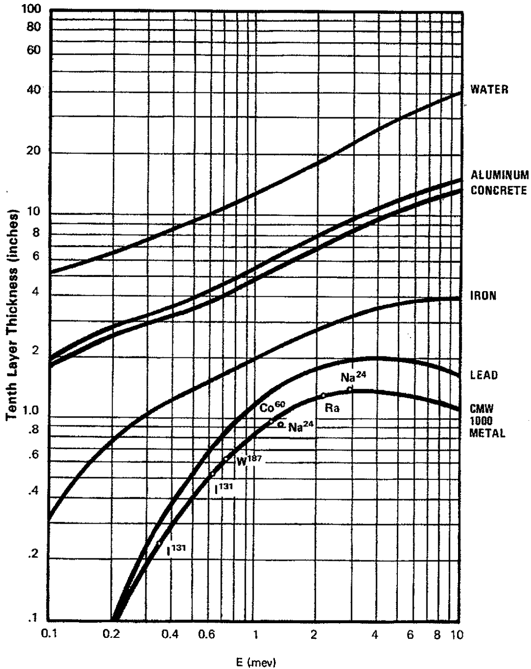
Gamma absorption characteristics of CMW ® 1000 and other shielding materials showing tenth layer thickness (narrow beam) radiation
