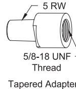
Tapered Adapter
